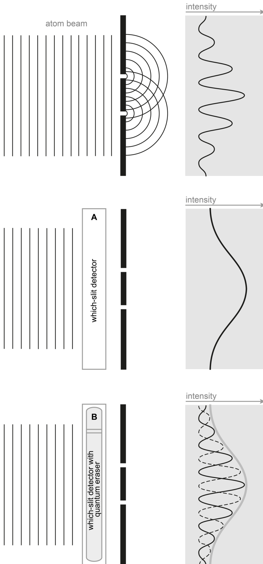
Figure 2: This set of diagrams illustrates some variations on a two-slit experiment. The source used in each case are atoms. The graphs to the right show the
