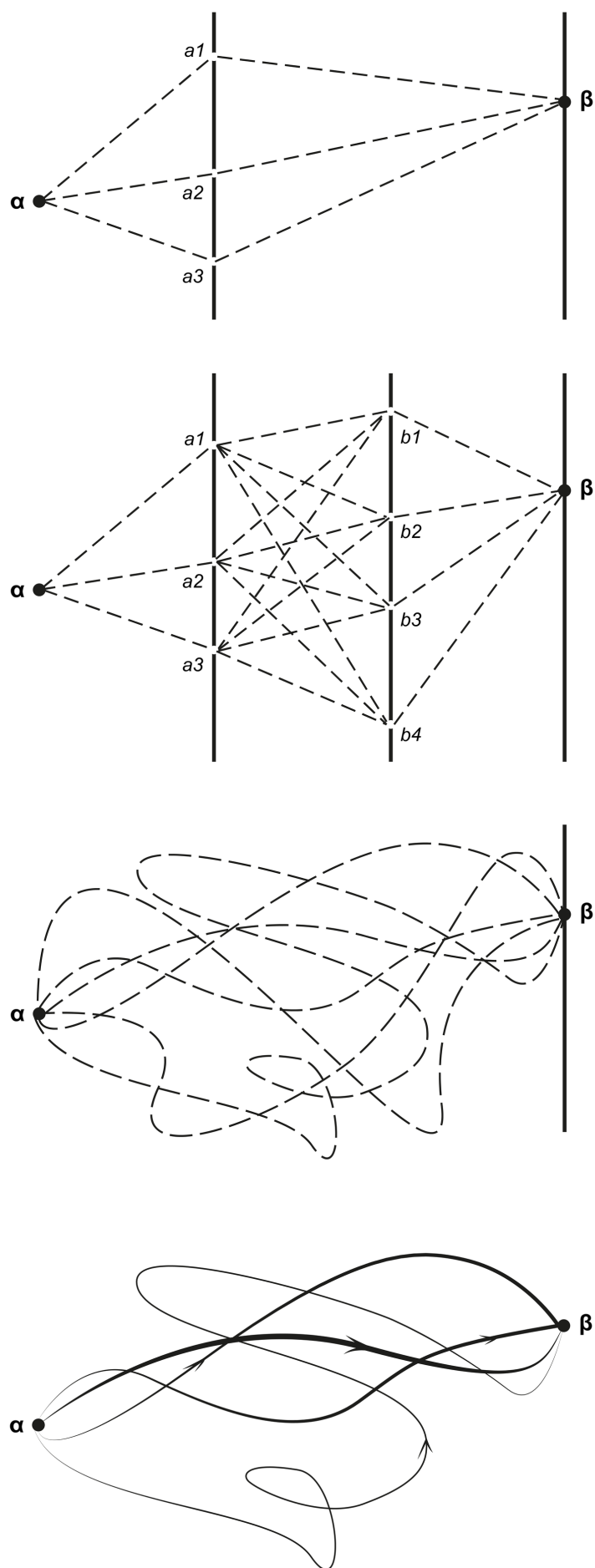
Figure 1: In these four diagrams, \alpha indicates the source of particles or the origin point, and \beta is a point on the screen marking the place where the
