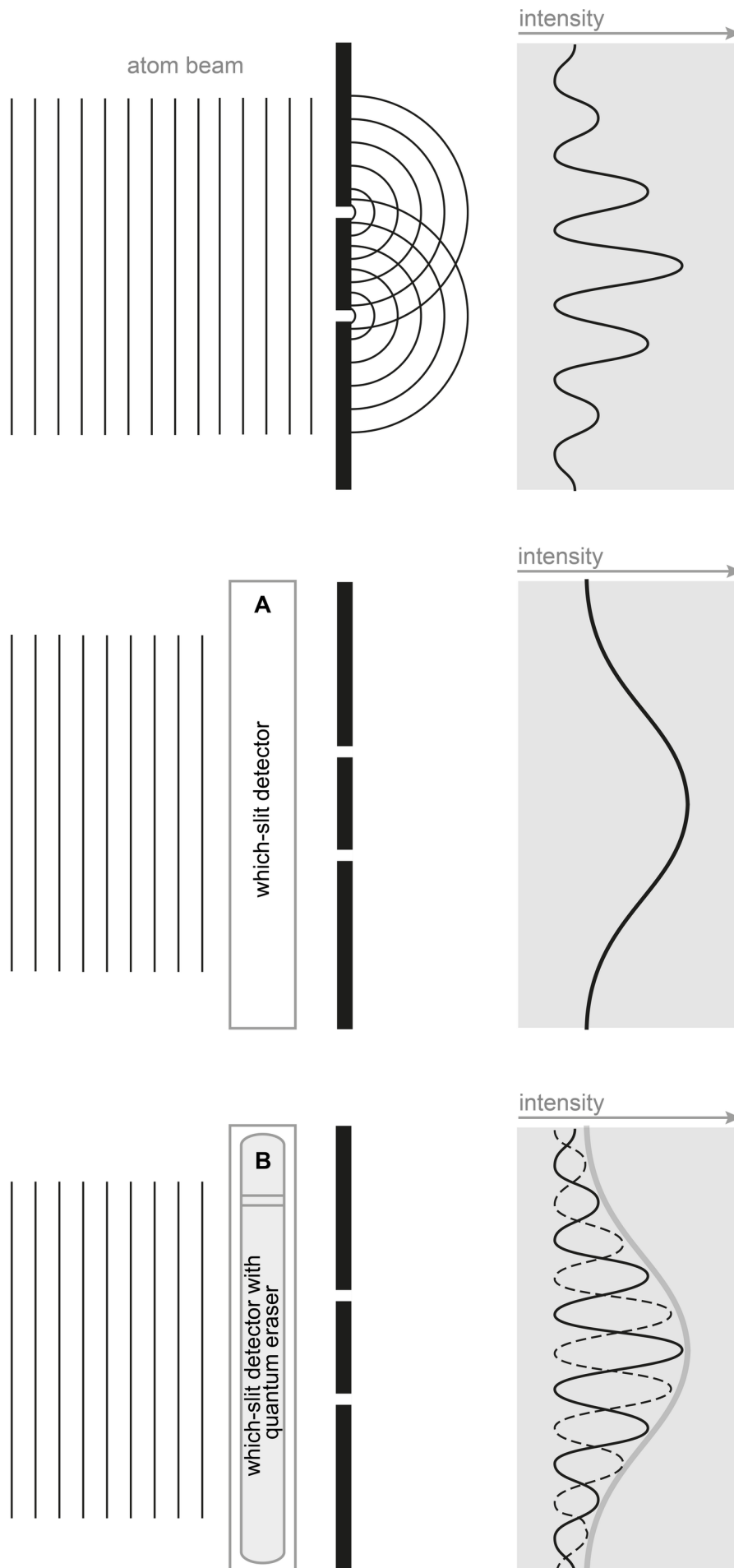
Figure 2: This set of diagrams illustrates some variations on a two-slit experiment. The source used in each case are atoms. The graphs to the right
